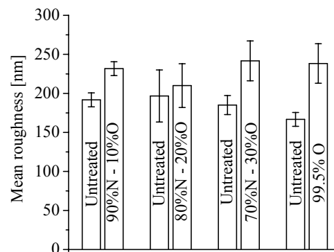
Figure 2. Mean roughness of the samples before and after the treatment.
