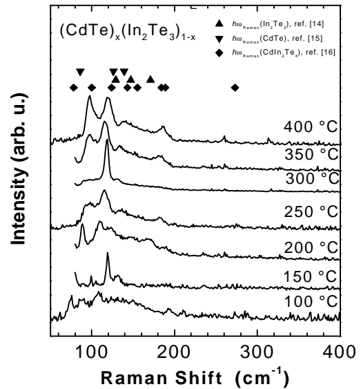
Fig. 2: Raman spectra as function of deposition temperature for the set of samples studied.
