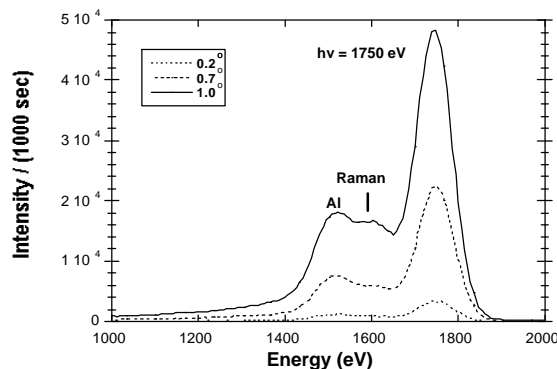
Fig. 4. Fluorescence spectra from a wafer intentionally contaminated with Al at a concentration of 8 x 10 12 atoms/cm 2 .
