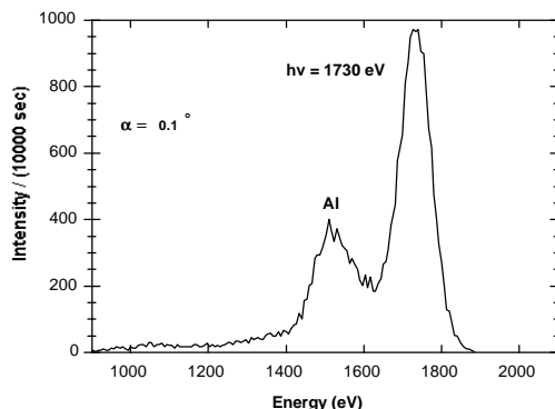
Fig. 5. Fluorescence spectra from a wafer intentionally contaminated with Al at a concentration of 3.4 x 10 9 atoms/cm 2 .
